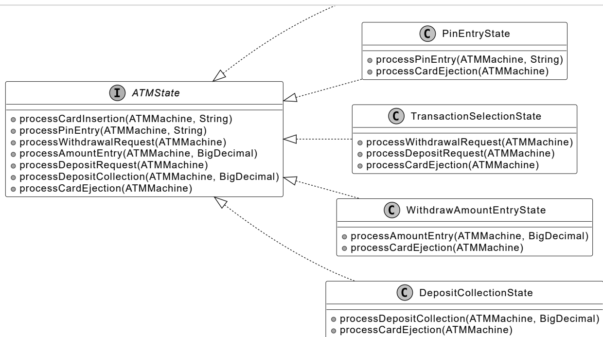
ATMState interface and concrete classes
