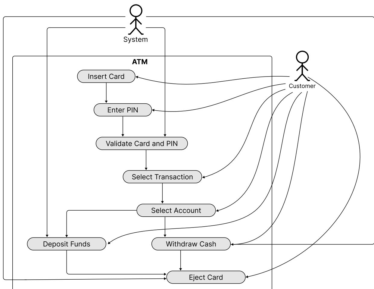
Use Case Diagram of ATM
